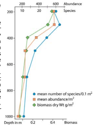
Figure 4-4 : Species richness, abundance and biomass of macrofauna along a radial on the continental slope in Crete (after Tselepidis & Eleftheriou, 1992).
