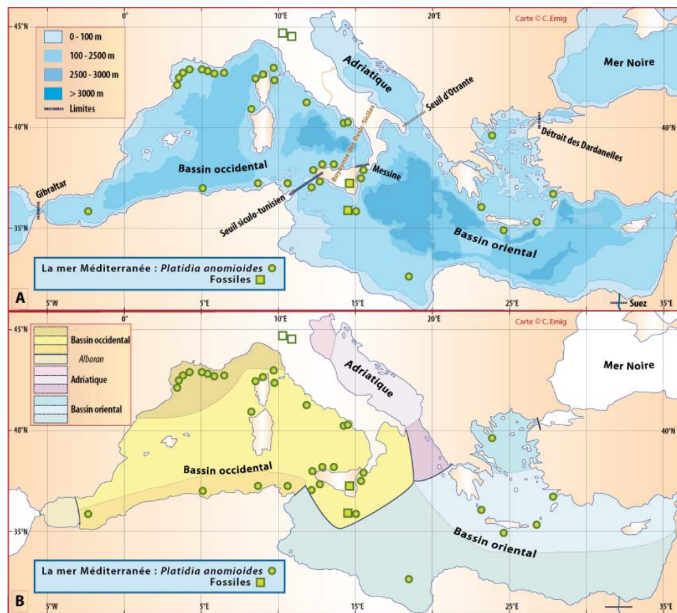
Figure 5-8 : Distribution of Platidia anomioides in the Mediterranean Sea, as well as reports of fossil forms. A. and B. _ see Fig 5-3 for basemap legend.
