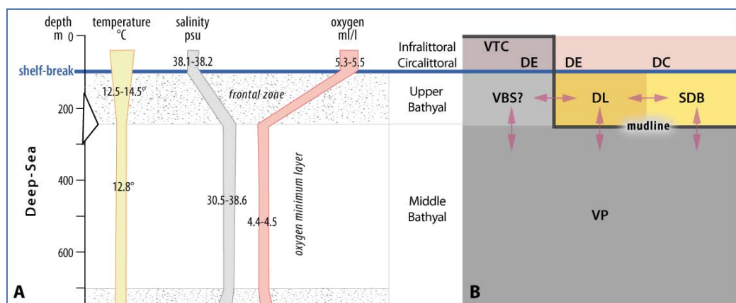
Figure 4-2 : A. Diagram of the different parameters of the water column in the Bathyal stage (from Emig, 1997a). B. Distribution of circalittoral and bathyal bioconoses along the continental slope with the limits and relationships of the benthic fauna. Bioconosis: DC - Coastal Detrital, DE - Silted Detrital, DL - Offshore Detrital, SDB - Bathyal Detrital Sands, VBS - Upper Bathyal Mud, VP - Deep Mud, VTC - Coastal Terrigenous Mud .
