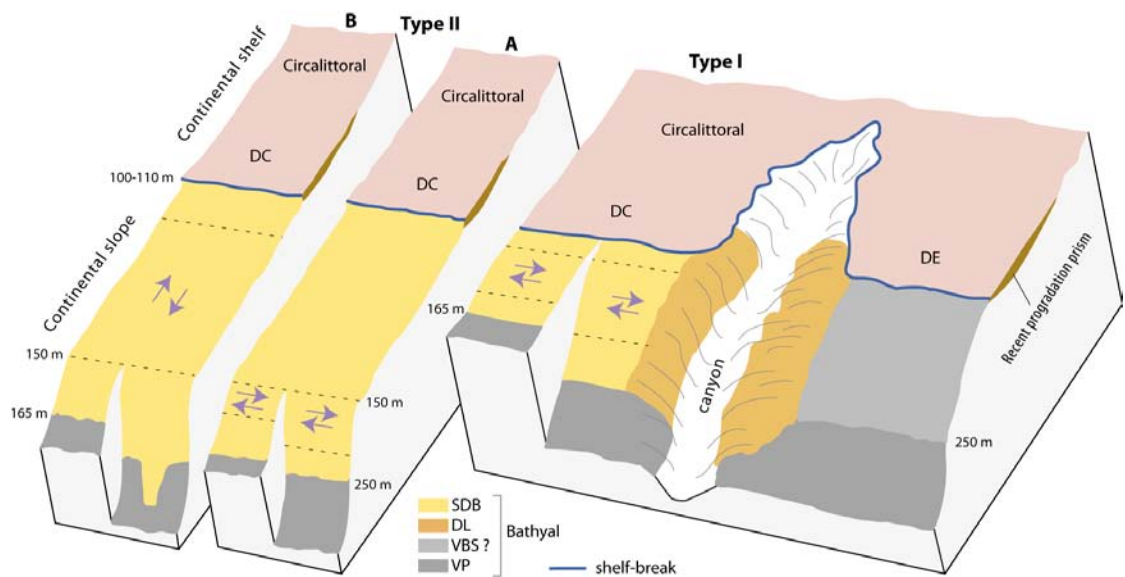
Figure 4-1 : Block diagram of the two main types of profile (I and II) of the upper zone of the Bathyal stage, with the distribution of the bioconoses, according to the slope and the depth (according to Emig, 1997a). The arrows indicate the direction of the bottom currents in the zones (between dotted lines) of maximum density of brachiopods where the currents are the most intense – see also Fig. 4-3. Bathyal bioconoses (see also Fig. 4-2): SDB = b. Bathyal Detrital Sands; DL=b. the Large Detrital; VBS = b. of the Upper Bathyal Vase; PV = b. of the Deep Vase. Circalittoral bioconoses: DC = b. Coastal Detrital; OF = b. Silted Detritus.
