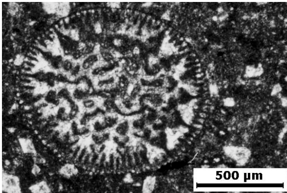
Figure 12: Thin section photograph. Montseciella arabica (somewhat oblique transverse section). Kharaiib (HST 3) in well N° 21.
