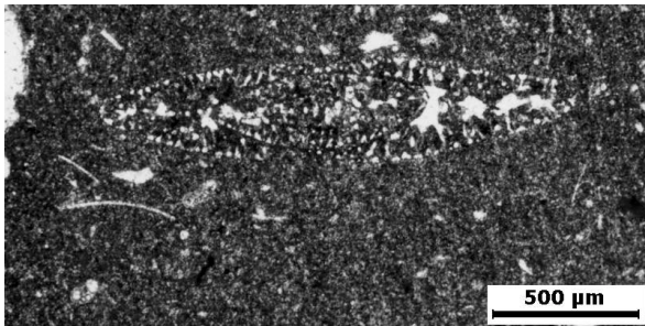
Figure 15: Thin section photograph. Hoffatella decipiens (subaxial section), along with planktonic foraminifera. Bab (LST 1) in well N° 21.
