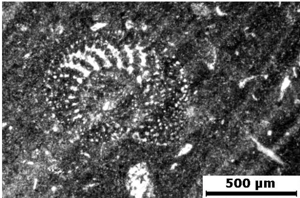
Figure 16: Thin section photograph. Hoffatella decipiens (equatorial section). Bab (LST 1) in well N° 21.
