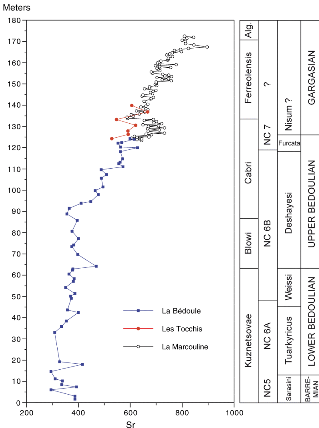
Figure 6: Evolution of Sr content in bulk carbonate in Bedoulian to Gargasian sediments from the Cassis area (La Bédoule, Les Tocchis and La Marcoulaine).
