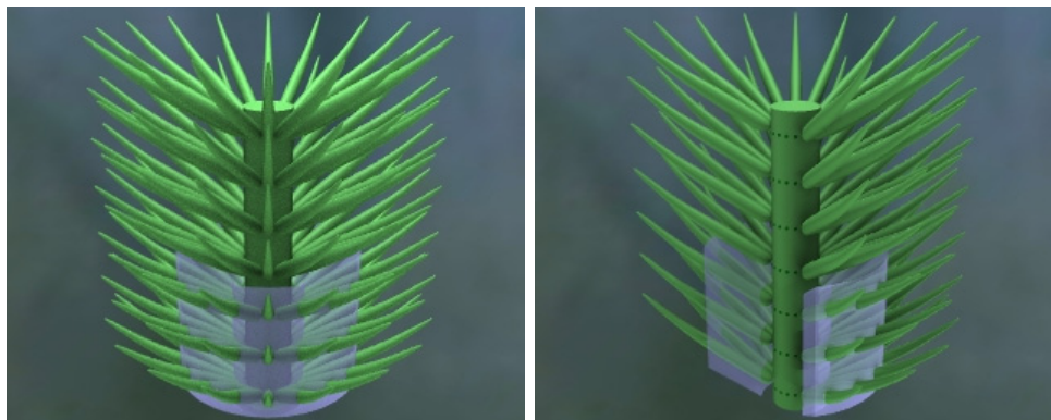
Figure 14: Reconstruction of Oligoporella prisca (like Pl. VIII, fig. 8).
