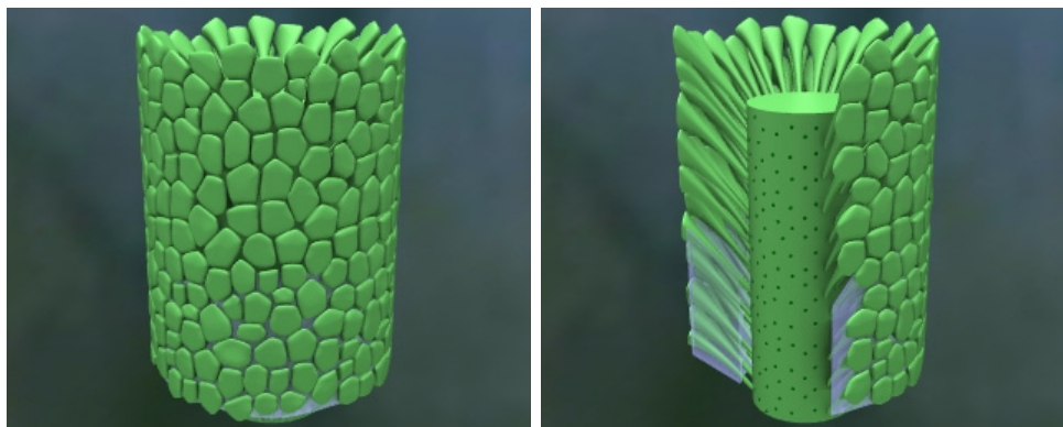
Figure 3: Reconstruction of Macroporella Bellerophontis (like Pl. VIII, fig. 8).
