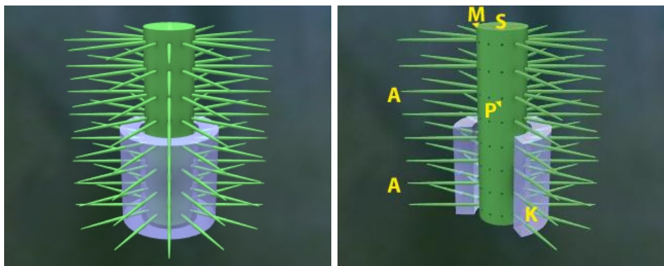
Fig. 8. General structural plan of the Diploporids
