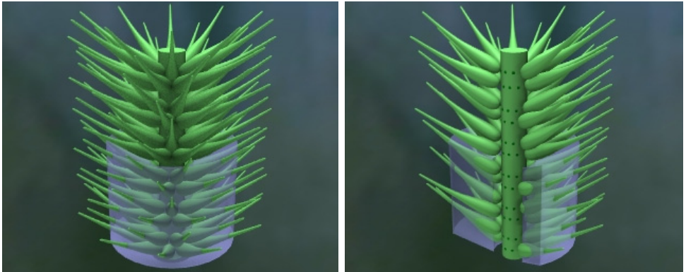
Figure 13: Reconstruction of Oligoporella serripora (like Pl. VIII, fig. 8).
