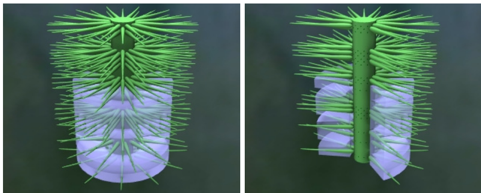
Figure 8: Reconstruction of Teutloporella vicentina var. nana (like Pl. VIII, fig. 8).
