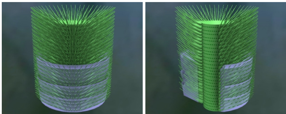
Figure 11: Reconstruction of Teutloporella triasina (like Pl. VIII, fig. 8).
