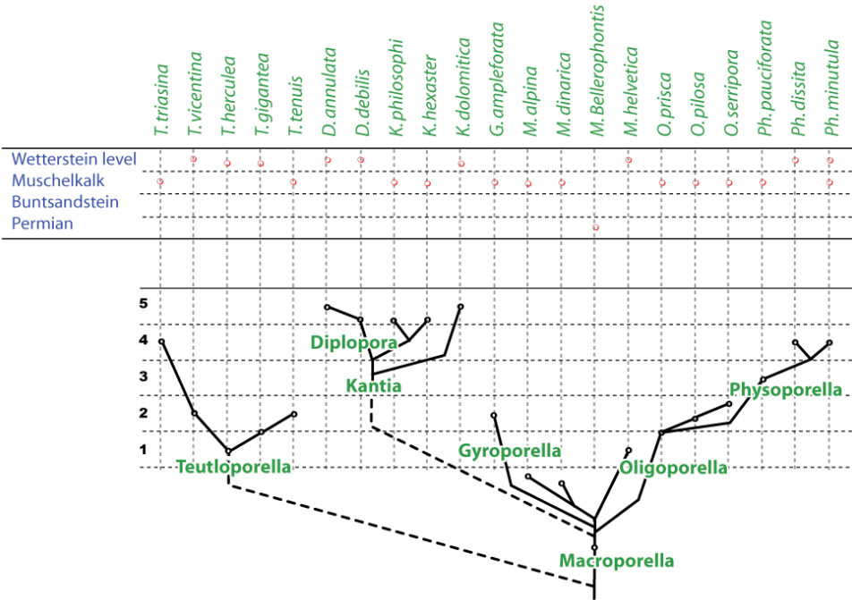
Figure 24: Tentative phyletic tree of the Diploporidae.
