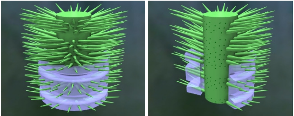
Figure 7: Reconstruction of Teutloporella vicentina (like Pl. VIII, fig. 8).
