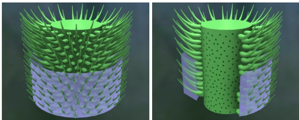
Figure 6: Reconstruction of Teutloporella gigantea (like Pl. VIII, fig. 8).
