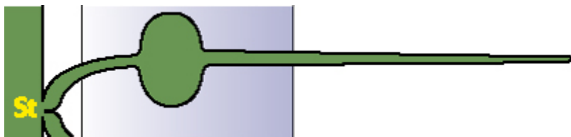
Figure 22: Longitudinal section through a branch of Diplopora annulata with a globular broadening (Sporangium?). St = main axis.
