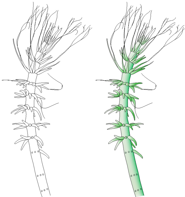
Fig. 9. Young sterile shoot of Neomeris annulata .
