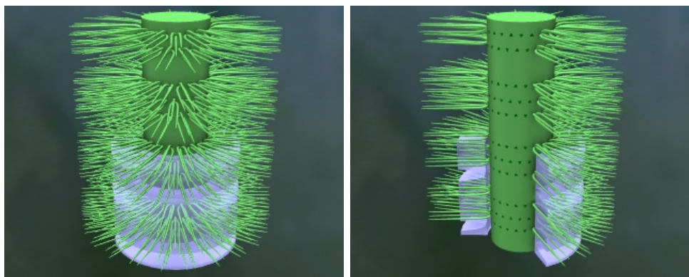
Figure 21: Reconstruction of Diplopora annulata (like Pl. VIII, fig. 8).
