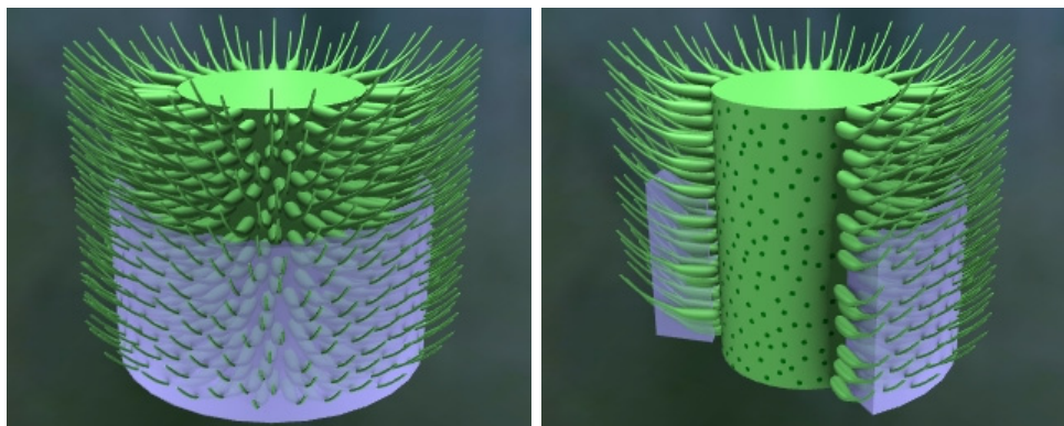
Figure 5: Reconstruction of Teutloporella herculea (like Pl. VIII, fig. 8).
