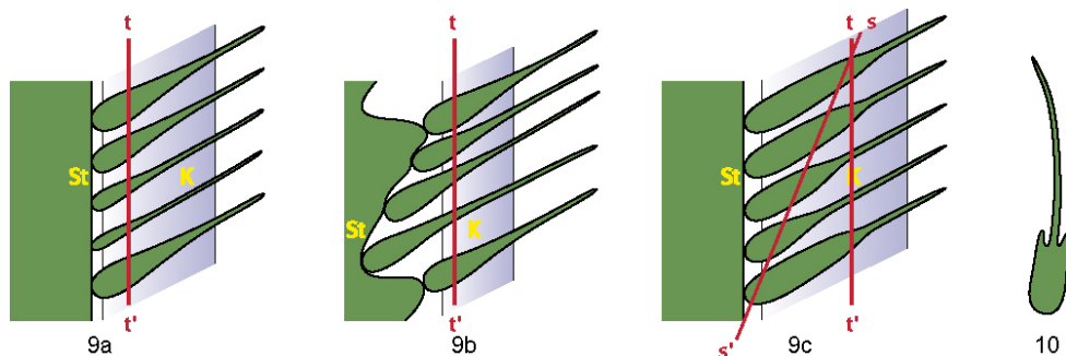
Figure 9a-c: Three possible interpretations for the tangential section of Teutloporella triasina . K = calcareous skeleton St = main axis [Stammzelle] t-t' = tangential section (Pl. IV, fig. 16) s-s' = oblique section (Pl. IV, fig. 15).
