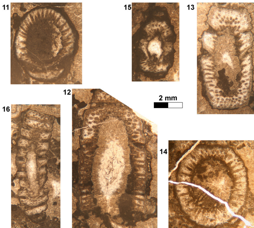
Figs. 11-14. Teutloporella vicentina TORNQUIST
