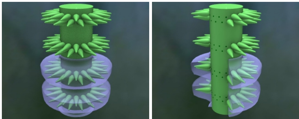
Figure 17: Reconstruction of Physoporella dissita (like Pl. VIII, fig. 8).
