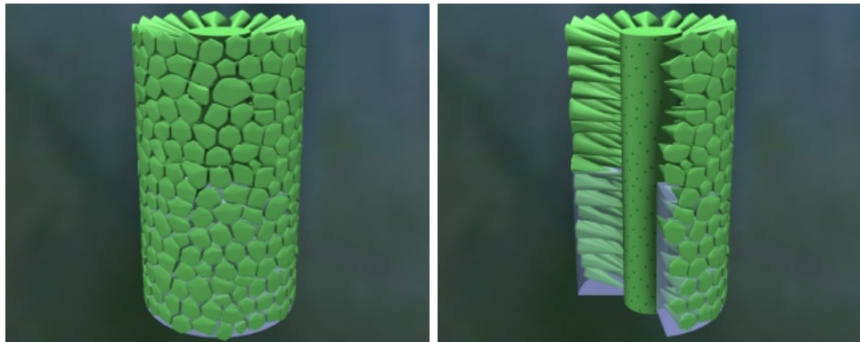
Figs. 10-16. Schematic generic reconstructions
