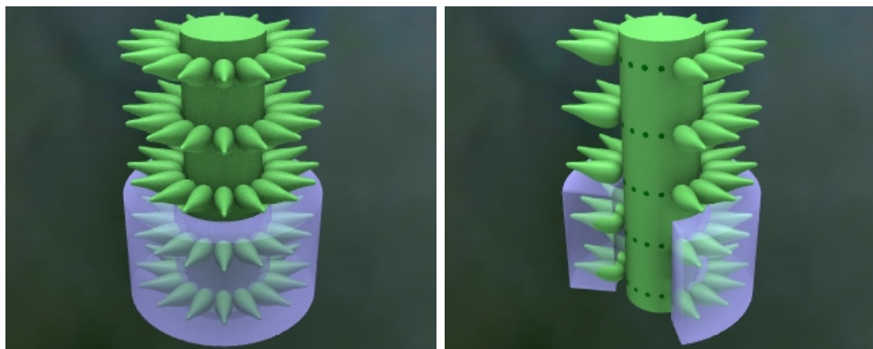
Figure 16: Reconstruction of Physoporella pauciforata (like Pl. VIII, fig. 8).
