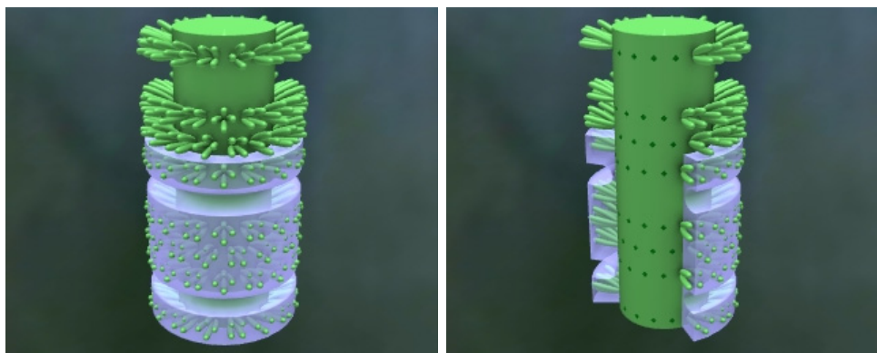
Figure 19: Reconstruction of Kantia philosophi (like Pl. VIII, fig. 8).
