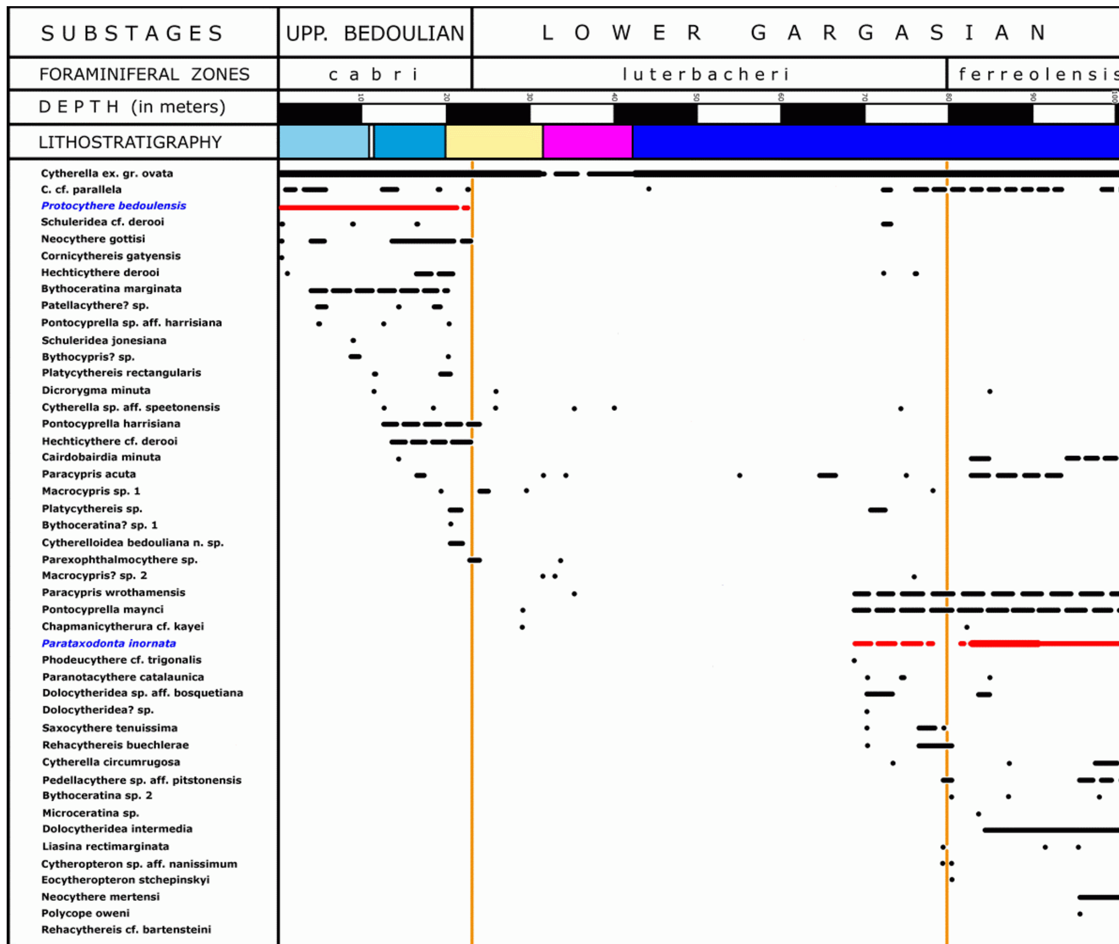
Figure 7: Composite distribution of Ostracoda in the upper Bedoulian-Lower Gargasian of the area of La Tuilière.
